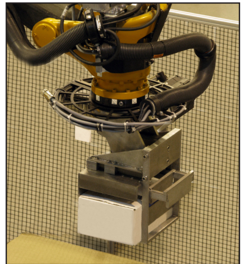
End-Of-Arm Tooling picking up a case
