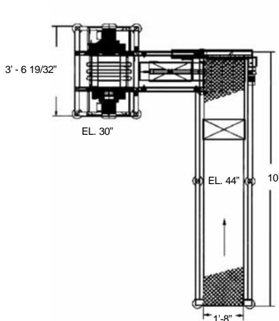
Original Right Angle Denester
