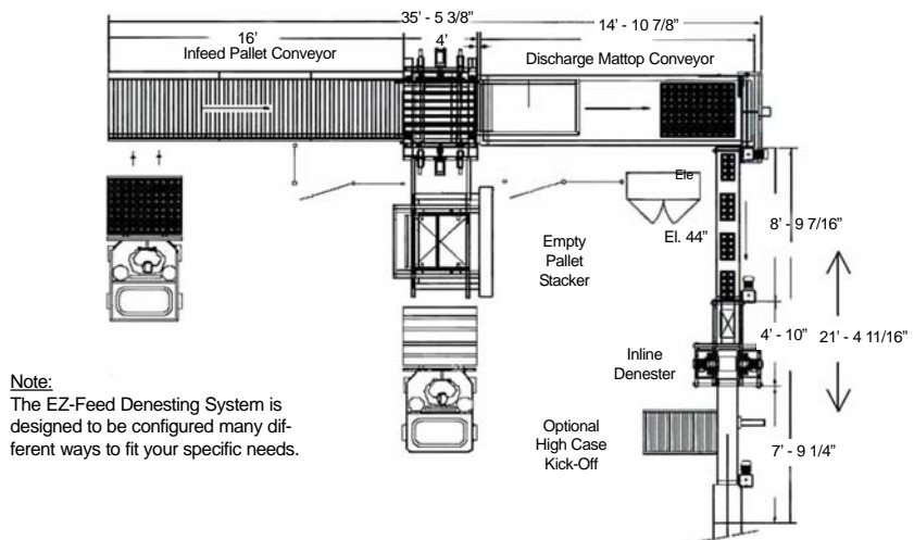
Automatic Returnable Shell Depalletizer/Denester System
